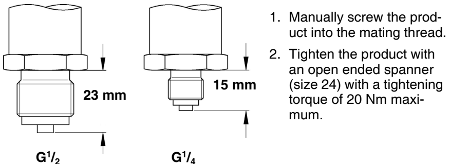
Fig. 2: Connection as per EN 837
