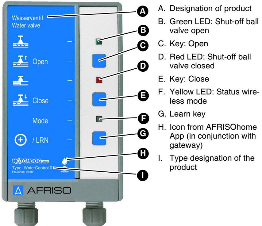
Fig. 1: Control unit
