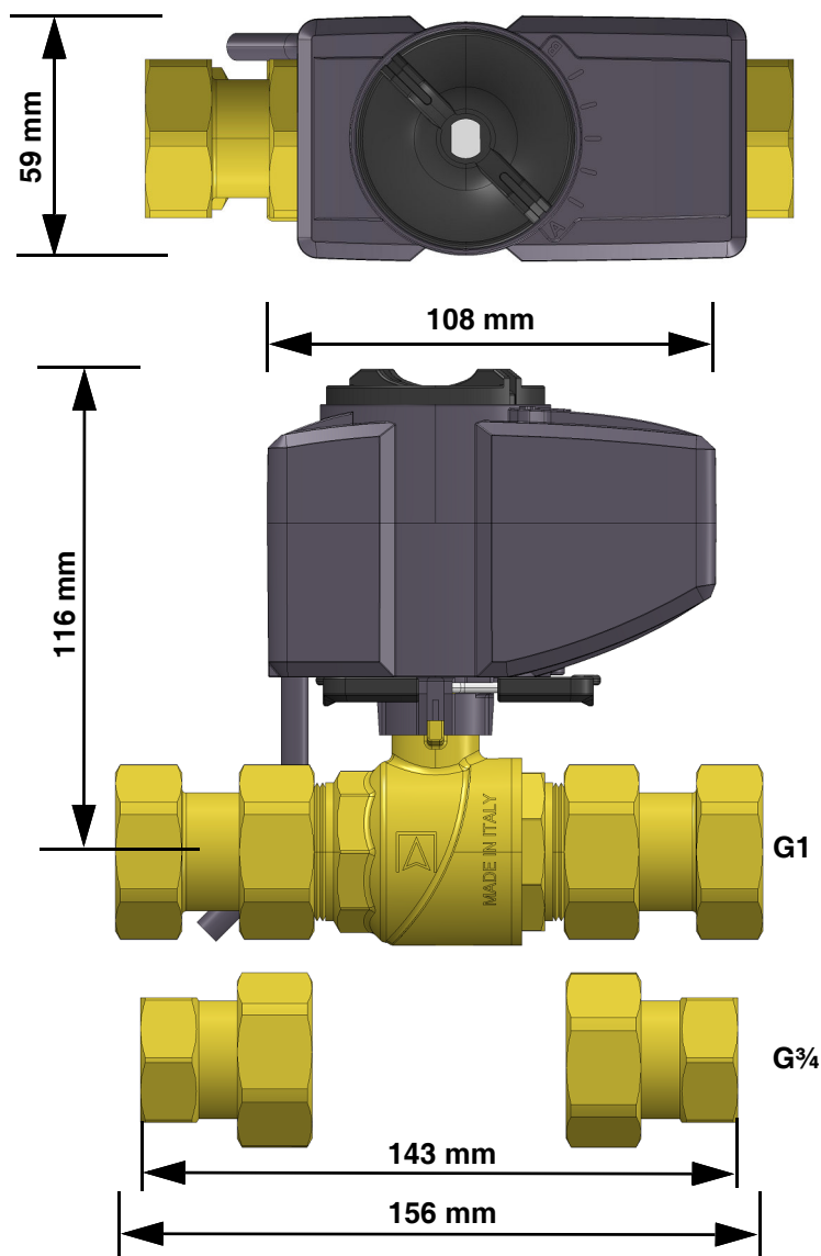
Fig. 3: Dimensions shut-off ball valve G1 with screw connections G \frac{3}{4} and G1
