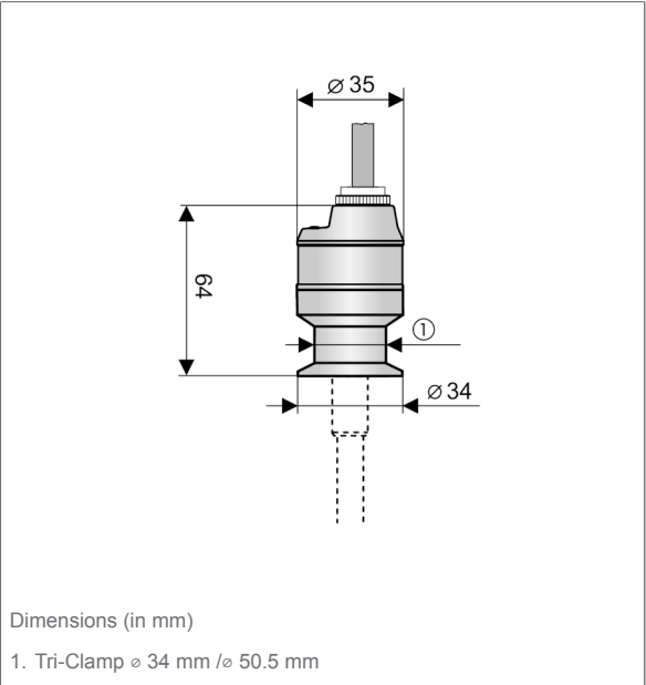
CapFox® EFT 20 with process connection Tri-Clamp DIN 32676
