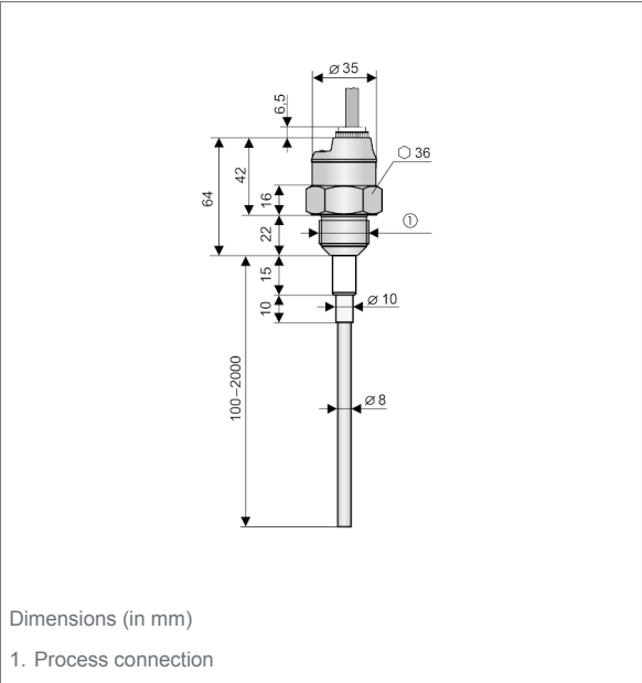
CapFox® EFT 20 MS - 21 with rigid mono probe with FEP insulation – CapFox® EFT 20 MS - 22 with rigid mono probe with PFA insulation
