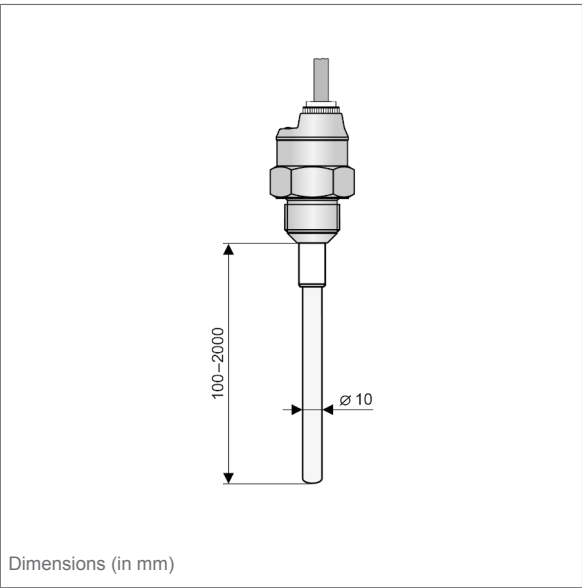
CapFox® EFT 20 MS - 21 with rigid mono probe with FEP insulation – CapFox® EFT 20 MS - 22 with rigid mono probe with PFA insulation
