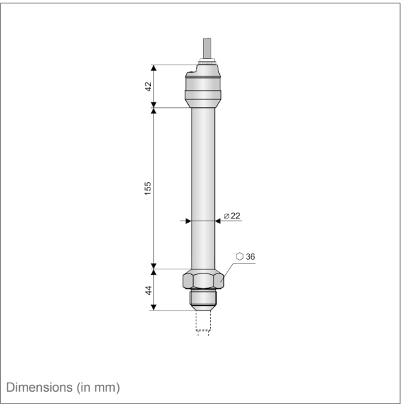
CapFox® EFT 20 high temperature version
