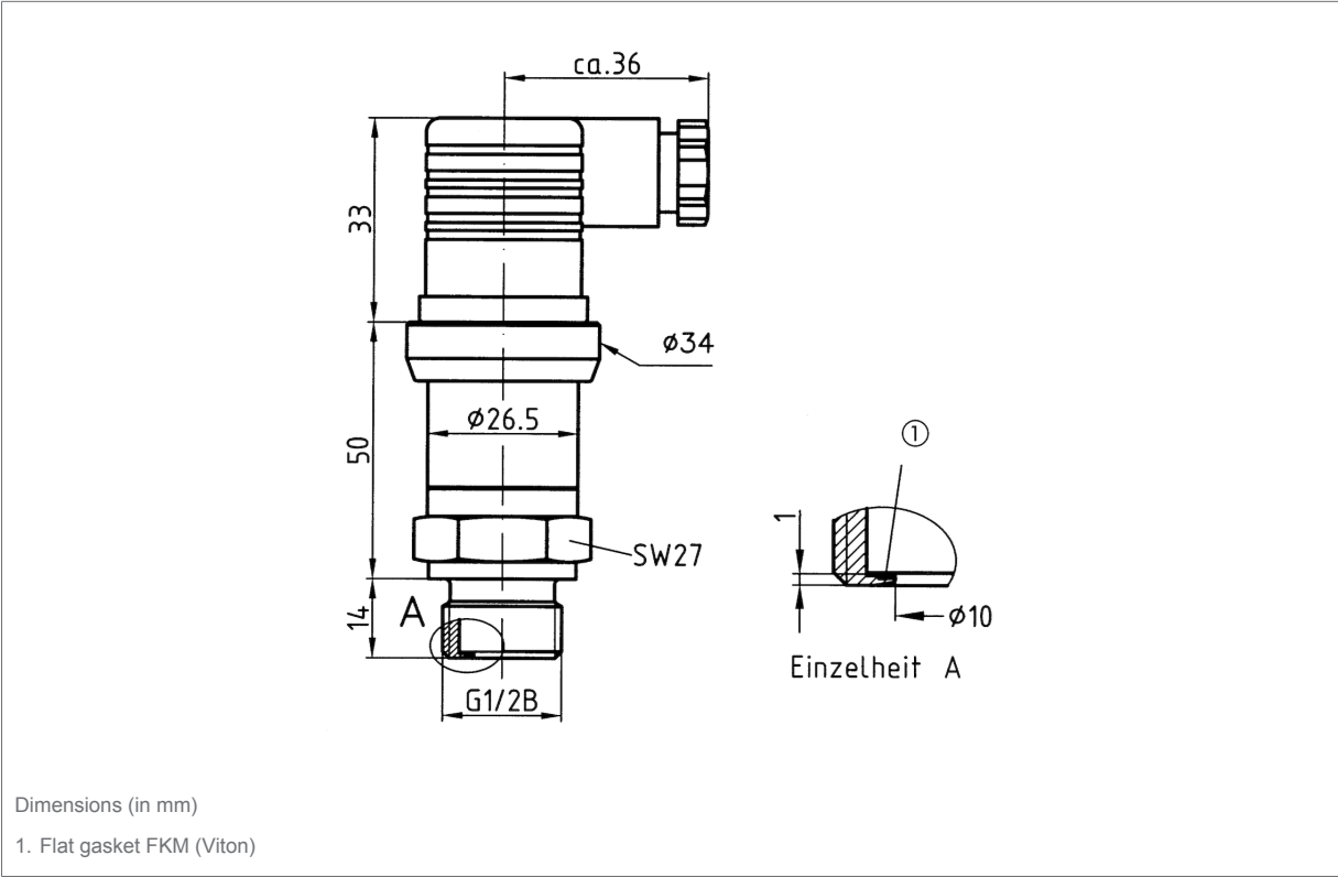
DMU 01 VM with connection G½B DIN 3852 type E with protruding diaphragm
