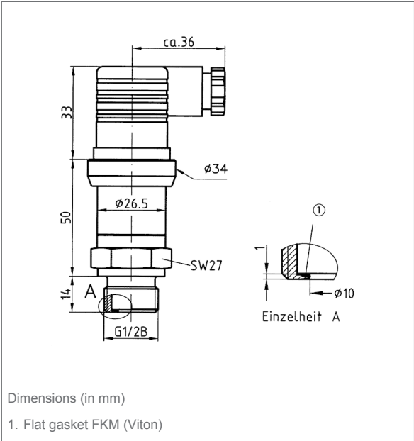
DMU 01 VM with connection G½B DIN 3852 type E with protruding diaphragm
