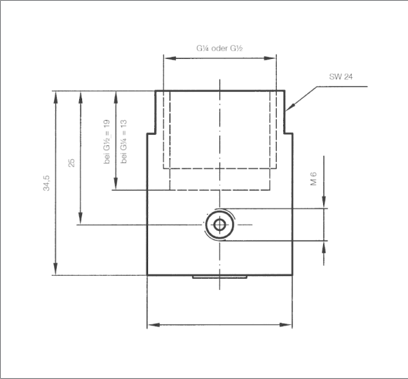
Adapter for instrument connection G¼/G½ with filling port
