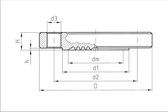
Type MD 80 - flange connection as per ASME B 16.5 (Raised Face)
