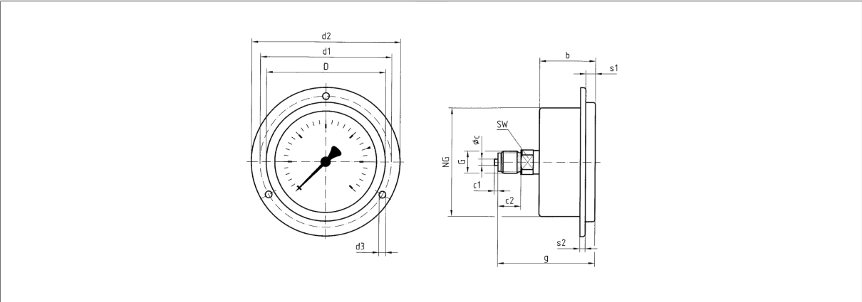
Dimensions (mm)
