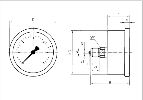
Dimensions (mm)
