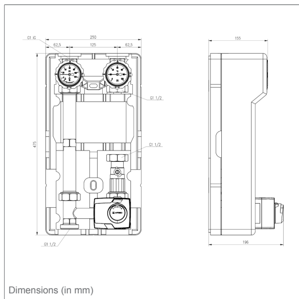
PrimoTherm® 180-2 without pump
