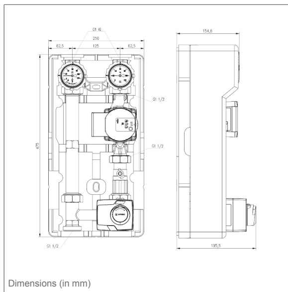
PrimoTherm® 180-2 with Wilo pump
