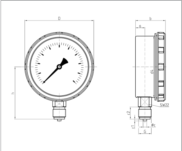
Dimensions (mm)
