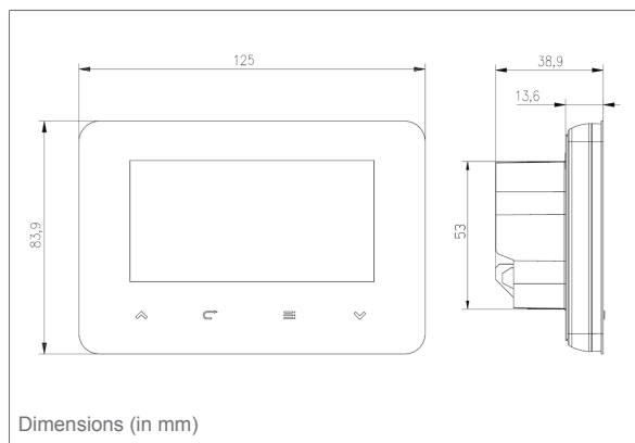
Room thermostat RT 05 D-230 / RT 05 D-BAT
