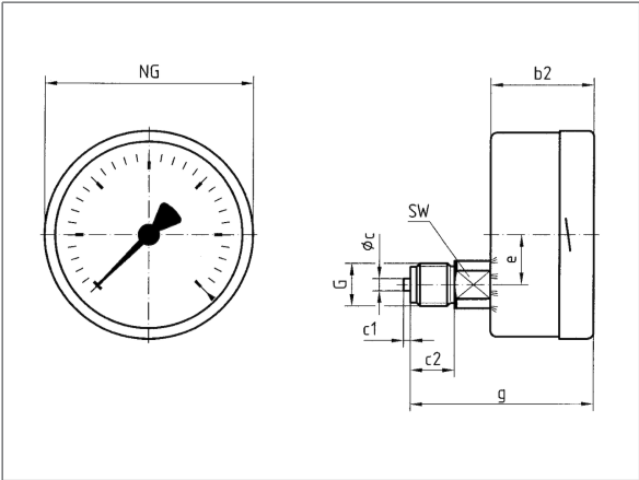
bottom back connection
