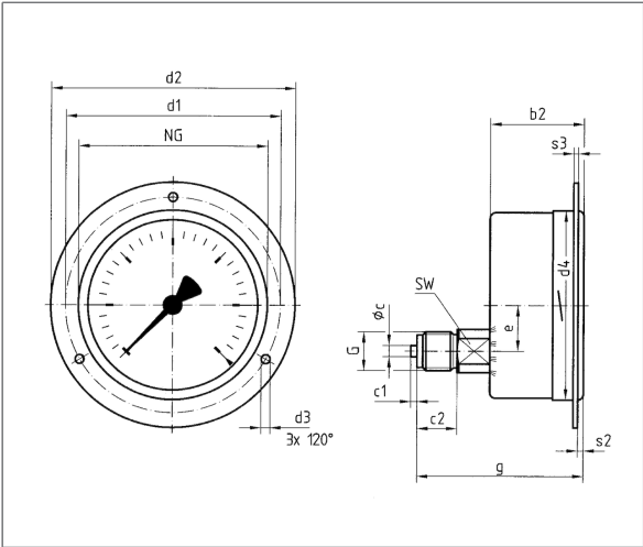
bottom back connection, 3-hole fixing, panel mounting bezel
