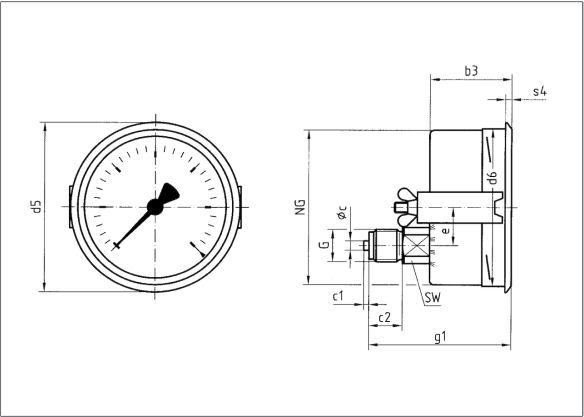
bottom back connection, panel mounting bezel with clamp fixing
