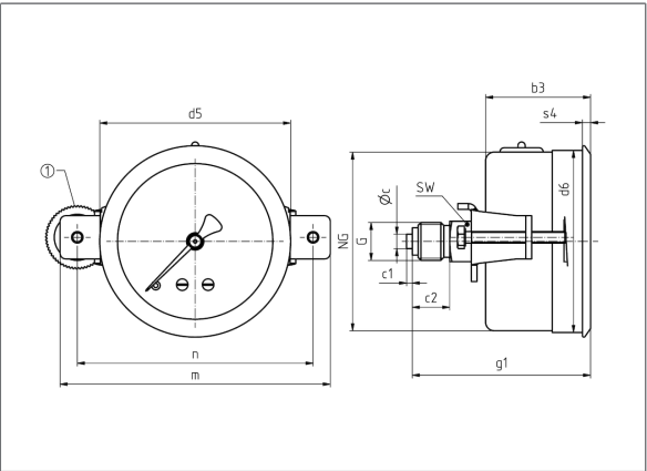
Centre back connection, panel mounting bezel with clamp fixing
