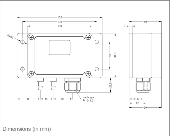
differential pressure transmitter DMU 20 D
