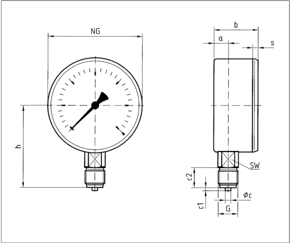
Dimensions (mm)
